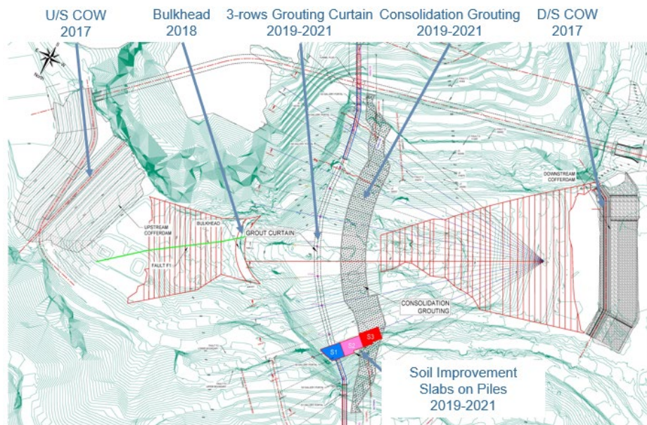
Fig. 9. The foundation engineering measures executed - general layout [1]
