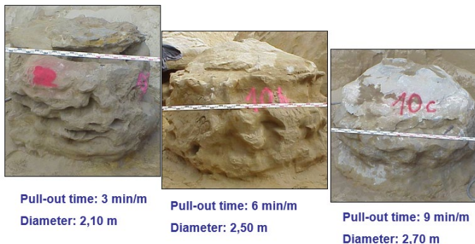
Fig. 8. Influence of retrieval rate on diameters achieved
